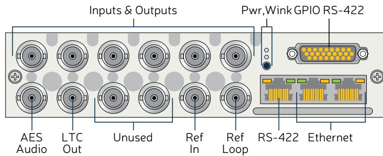
Six SDI I/O ports: two inputs, four outputs
